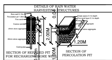
DETAILS OF RAIN WATER HARVESTING STRUCTURES
