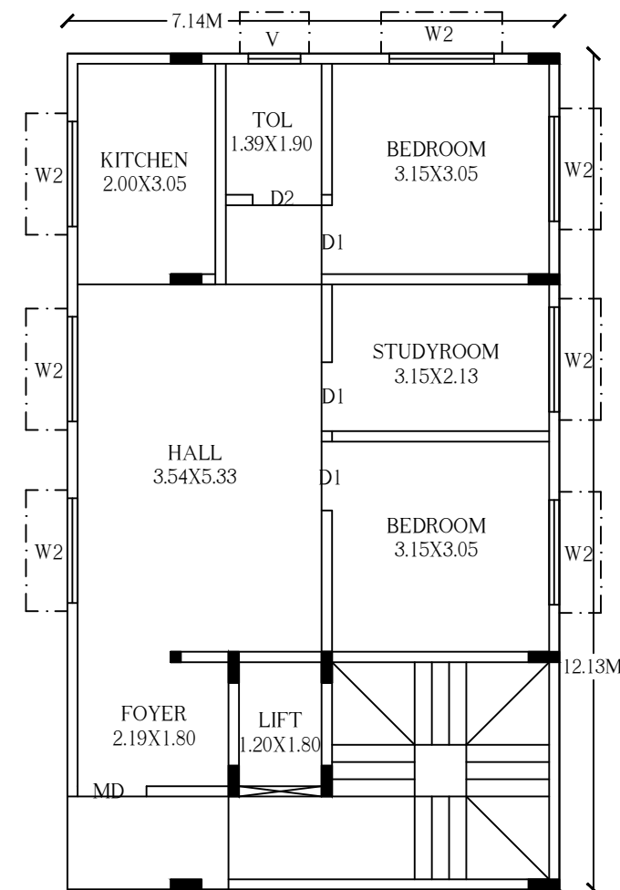
TYPICAL GROUND, FIRST & SECOND FLOOR PLAN
